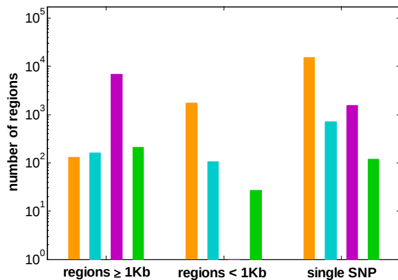
Simple merge - CNPs
