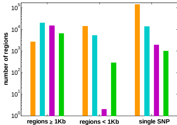
Simple merge - CNVRs
