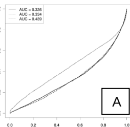
ROC curves
