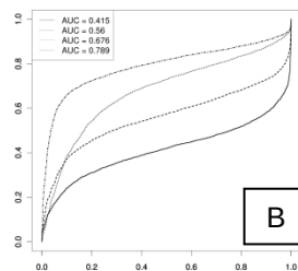
ROC curves
