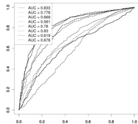
ROC curves
