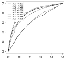
ROC curves
