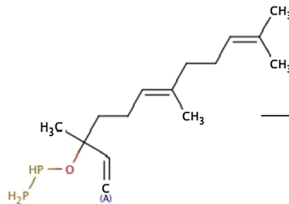
Nerolidol diphosphate
