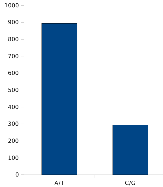
Frequencies of different SSR repeat motif types in mononuceotide
