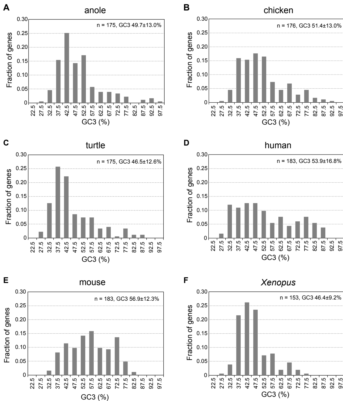
Additional file 4. GC 3 distribution of the orthologs in other vertebrates. Histograms show frequency distributions of orthologs in green anole lizard (A), chicken (B), Chinese soft-shelled turtle (C), human (D), mouse (E) and Xenopus tropicalis (F).
