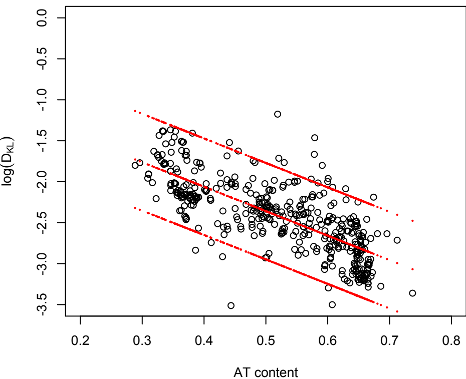
Phages
