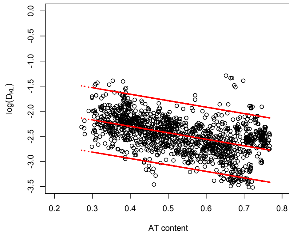
Plasmids
