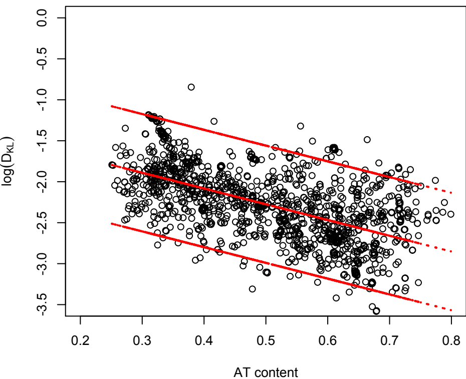
Chromosomes
