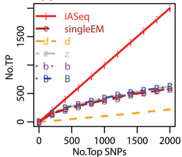
(a) Scenario 1: dataset 1
