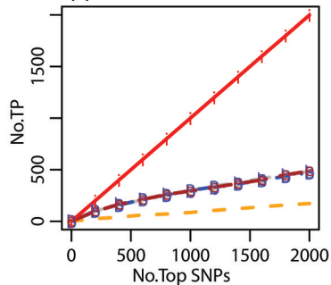
(c) Scenario 1: dataset 21
