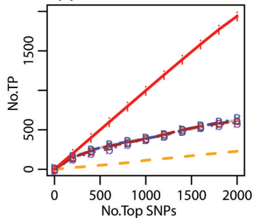
(e) Scenario 2: dataset 1
