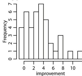
(h) Scenario 2: dAUC Hist.
