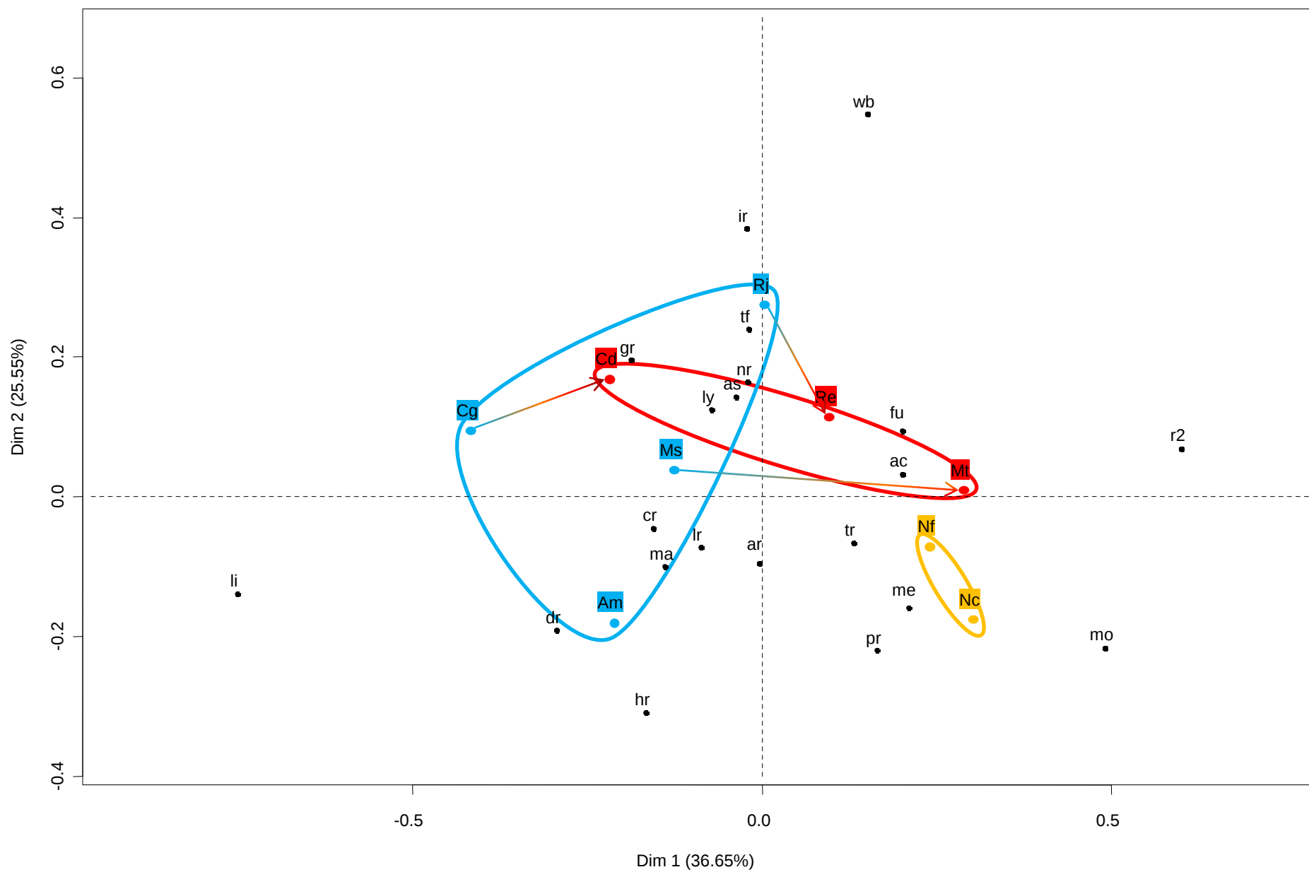
Transcription domains
