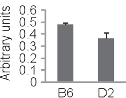
Lipid to protein ratio
