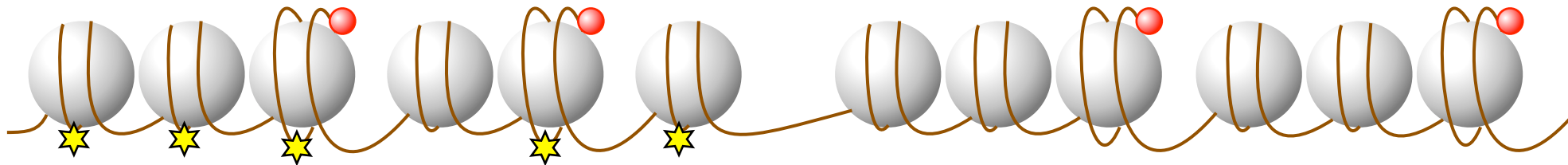
Sparse H4K5ac - Inactive gene
