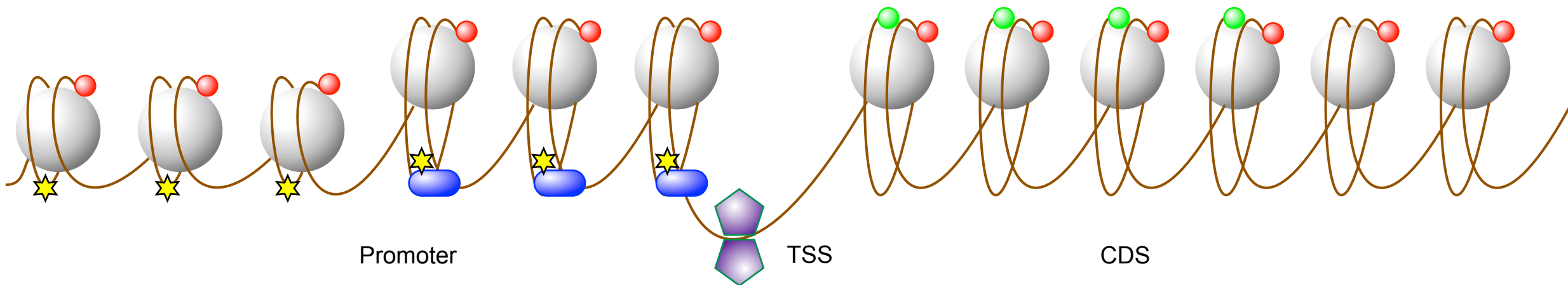
Hyperacetylated for H4K5 - Primed gene
