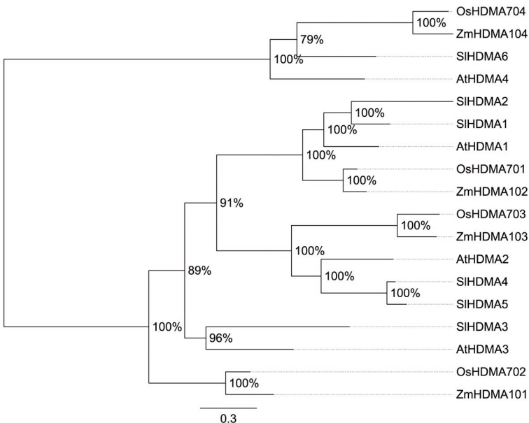
Additional file 9. Phylogenetic tree of HDMA proteins. Bayesian phylogenetic tree of HDMA predicted proteins from Arabidopsis thaliana (At), Oryza sativa (Os), Solanum lycopersicon (Sl) and Zea mays (Zm). Bootstrap values higher than 50% are shown. The tree is drawn to scale, with branch lengths measured in the number of substitutions per site.
