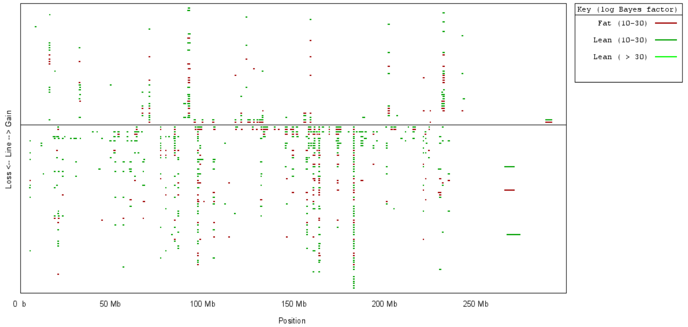
Titan Chromosome 1
