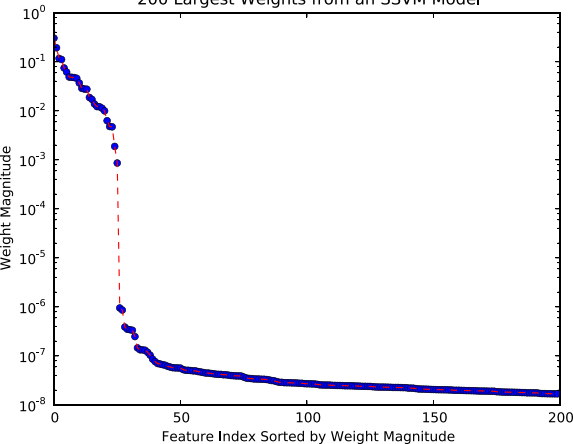
200 Largest Weights from an SSVM Model
