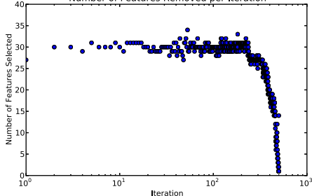
Number of Features Removed per Iteration
