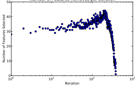
Number of Features Removed per Iteration
