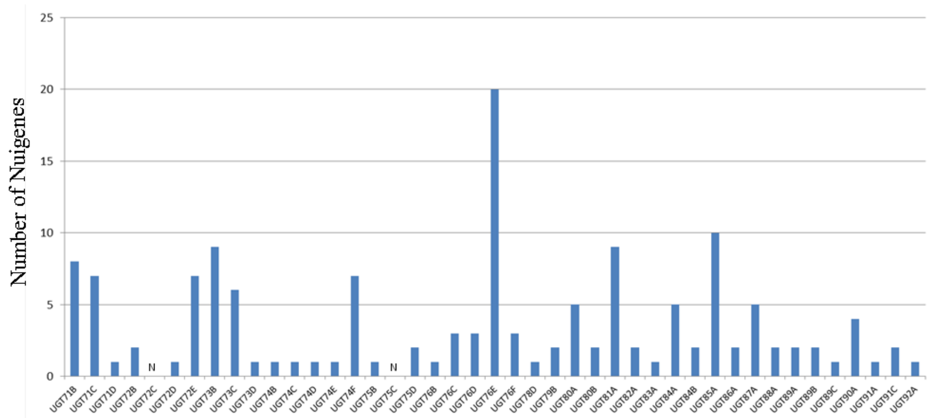
Additional file 11 The contribution of 41 UDP-dependent glycosyl transferases families in I. indigotica . UGT72C and UGT75C families were not found in I. indigotica transcriptome.
