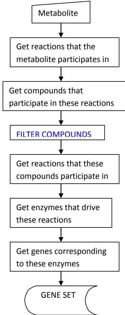
B. Reaction Scheme
