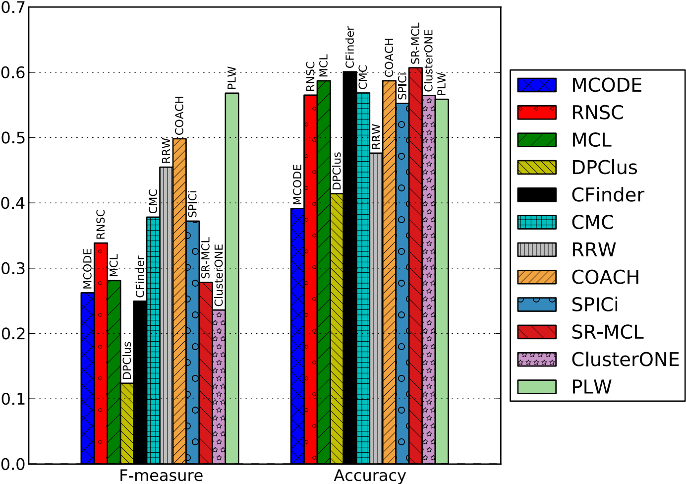
Supplementary File 4 - Performance of algorithms on COMBINED6 data against NEWMIPS gold standard
