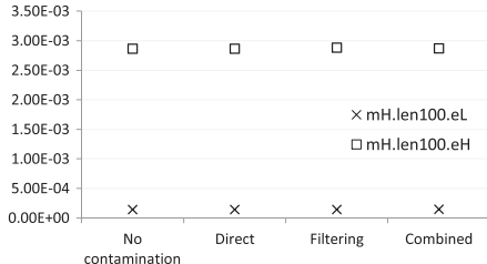
False negative rate
