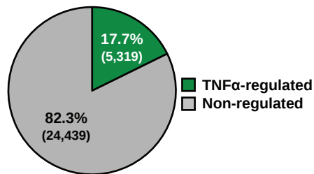
A All Expressed Transcripts
