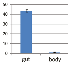
P450 CYP6 family (CL450.Contig1)
