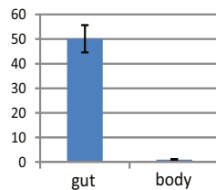
P450 CYP6 family (Unigene744)
