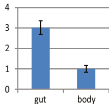
P450 CYP4 family (Unigene8300)
