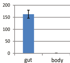
P450 CYP4 family (CL569.Contig2)
