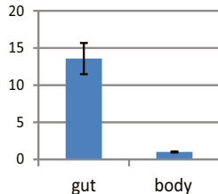
Trehalose transporter (CL165.Contig2)
