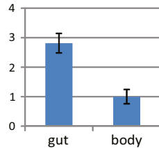
Trehalose transporter (Unigene6684)
