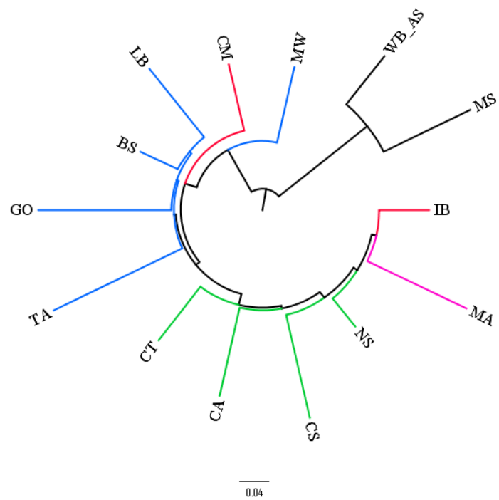
Dendrogram based on F_{st} pairwise between local breeds using 60K data
