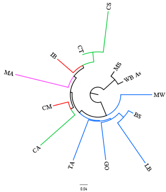
Dendrogram based on F_{st} pairwise between local breeds using 16.409 non-synonymous sites
