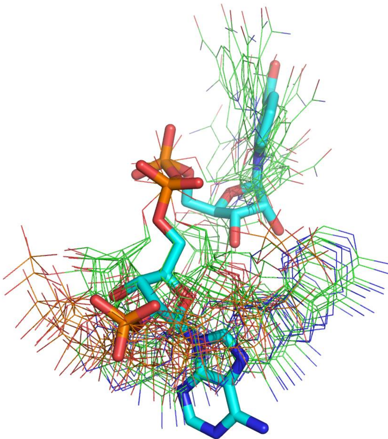
Supplementary Figure 8: Conformers of NADP molecule used for RosettaLigand Dock analysis. Molecule in 'sticks' (cyan) is borrowed from crystal structure 2JL1. Another 884 conformers (green lines) were generated by sampling 13 rotatable dihedrals \pm 30^\circ from the dihedrals found in crystal structure.
