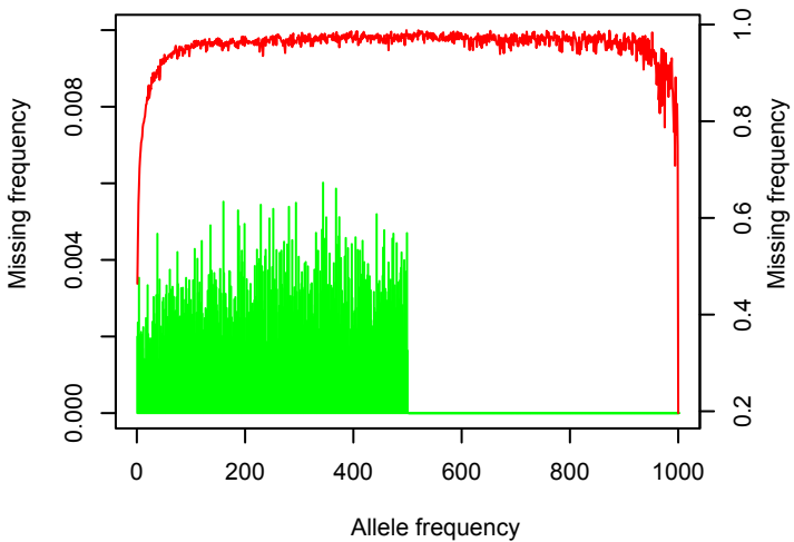
Chromosome 13
