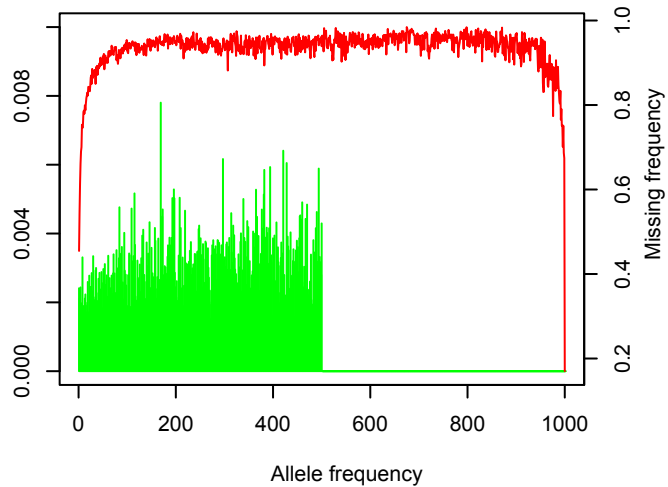
Chromosome 14
