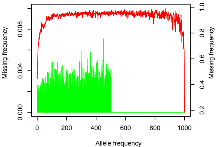
Chromosome 16
