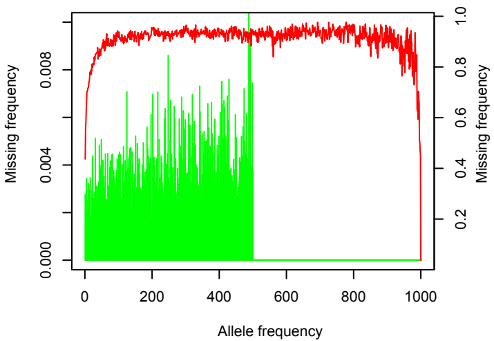
Chromosome 19
