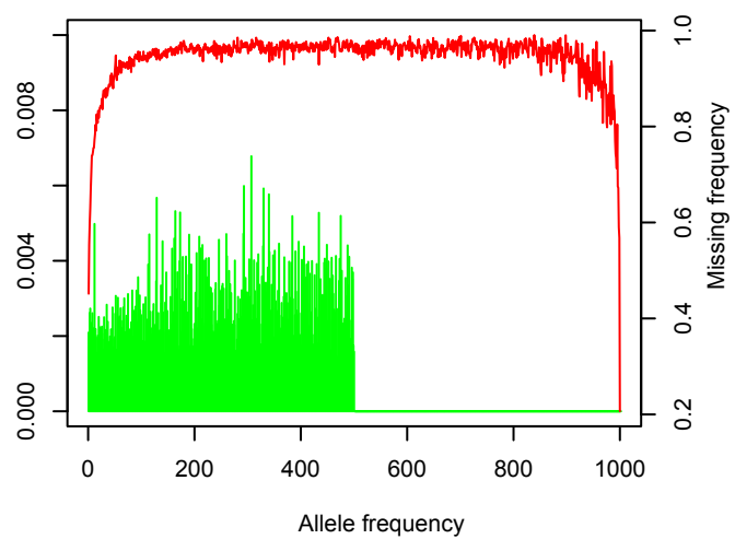
Chromosome 20
