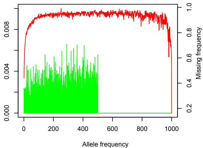
Chromosome 17
