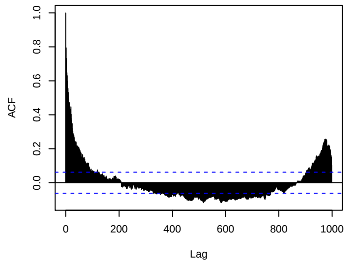
Chromosome 17
