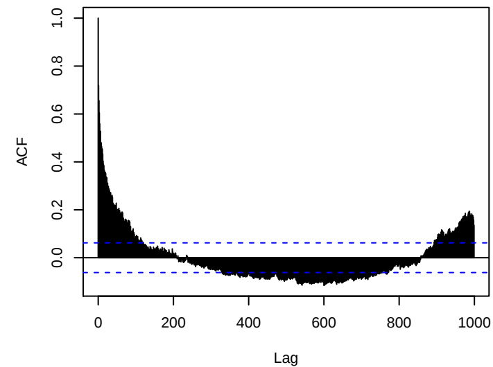
Chromosome 18
