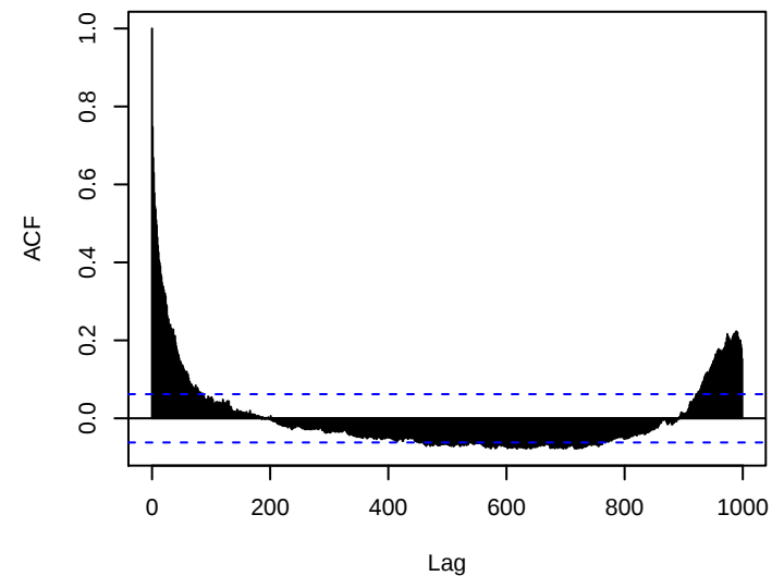
Chromosome 6
