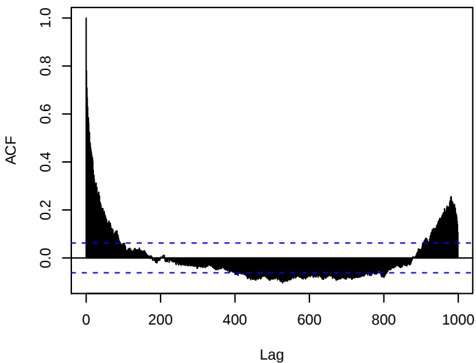
Chromosome 16
