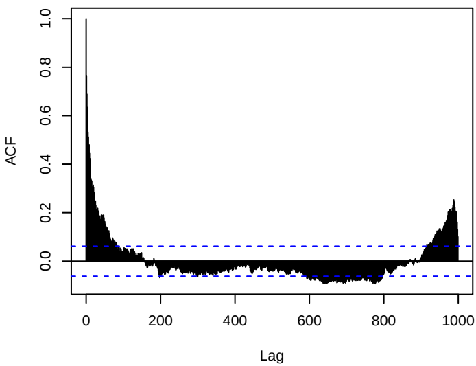
Chromosome 19
