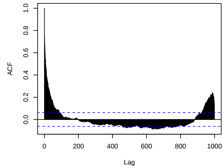
Chromosome 12
