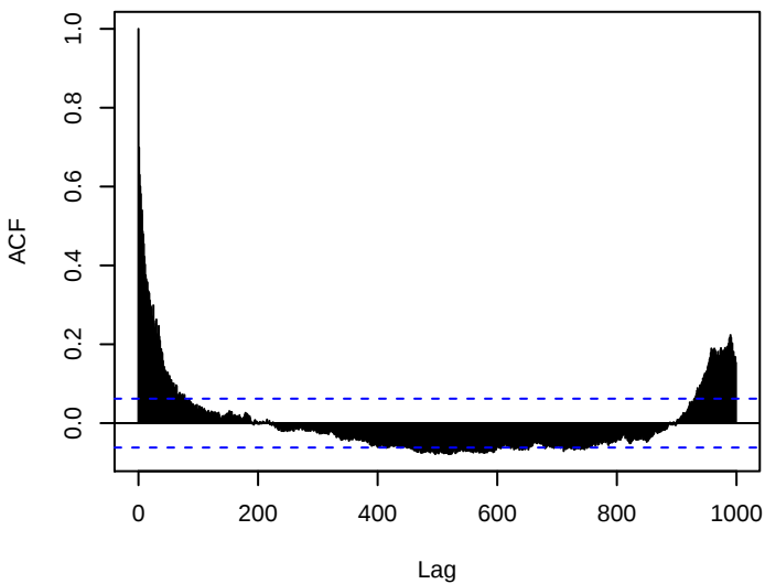
Chromosome 16
