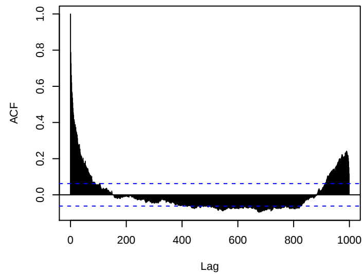
Chromosome 20
