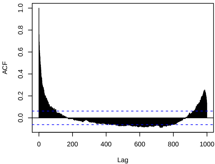
Chromosome 10
