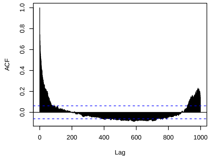
Chromosome 11
