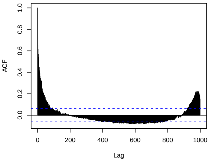
Chromosome 10
