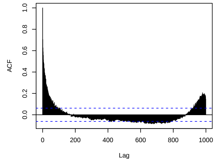
Chromosome 18
