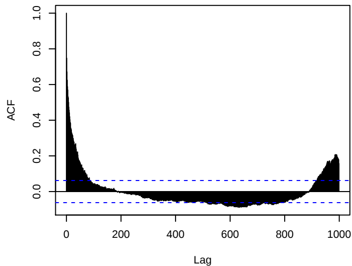
Chromosome 5
