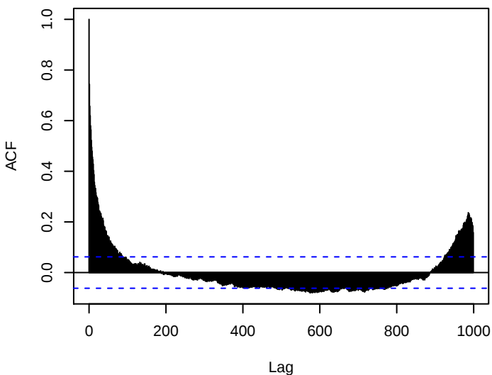
Chromosome 4
