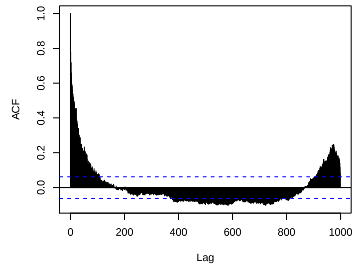
Chromosome 21
