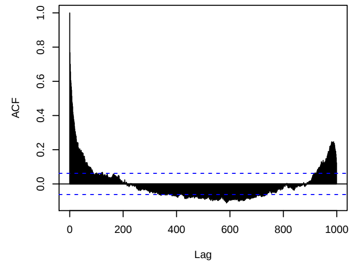
Chromosome 12
