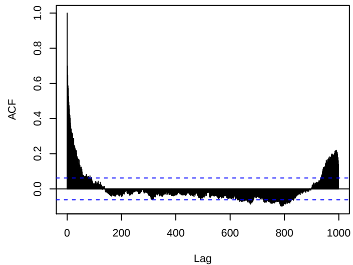
Chromosome 17
