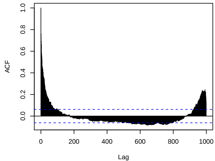
Chromosome 11
