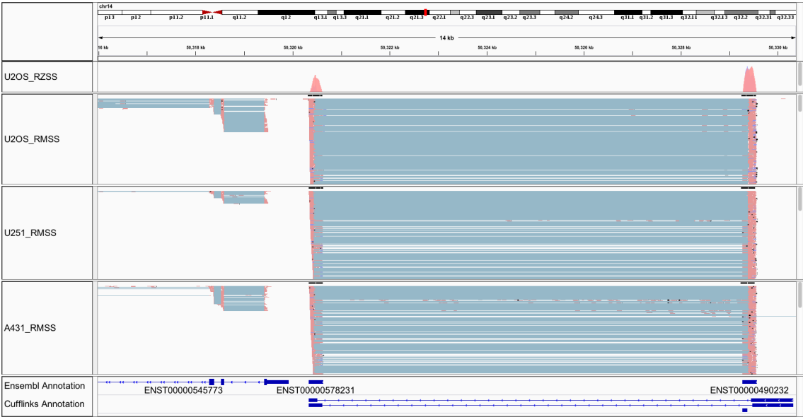
Figure S7: Ubiquitous transcription on chromosome 14 suggests fault in current annotation. As shown in the annotation tracks at the bottom of the figure, this loci is annotated as two genes in Ensembl (ENST00000578231 and ENST00000490232). Our data suggests that these are two exons of the same gene as shown by the inserts in the read data and the Cufflinks annotation track.
