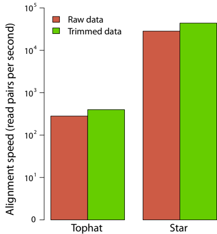
Alignment speed for raw data and trimmed data
