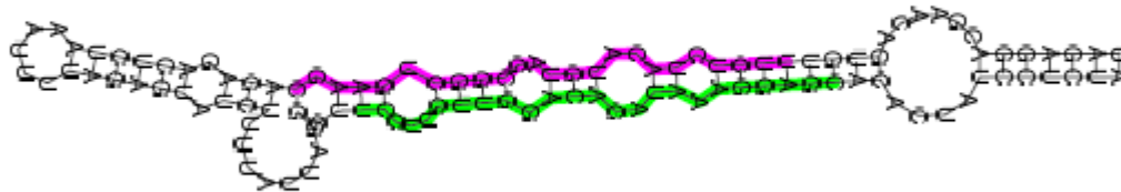
Zma_miR_Seq11_chromosome1 _7827584_7827607
