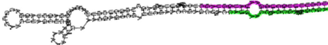
Zma_miR_Seq12_chromosome6 _107369829_107369852
