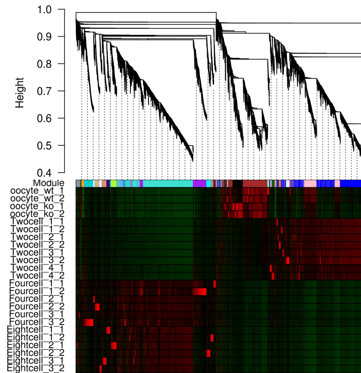
A Cluster Dendrogram
