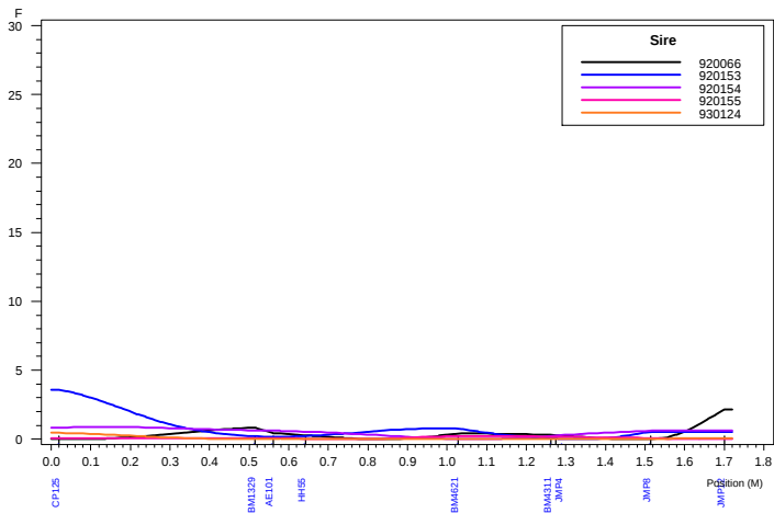
Haley-Knott QTL Analysis: Chromosome 6 LIGE
