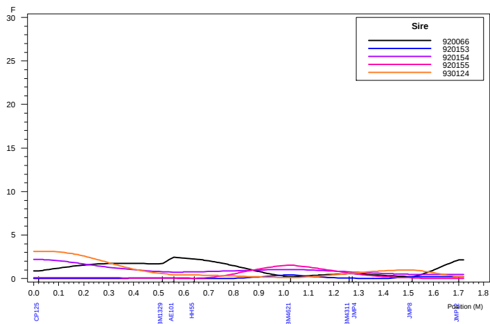
Haley-Knott QTL Analysis: Chromosome 6 DAG2
