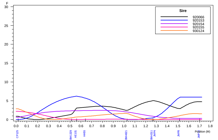
Haley-Knott QTL Analysis: Chromosome 6 ELISA5
