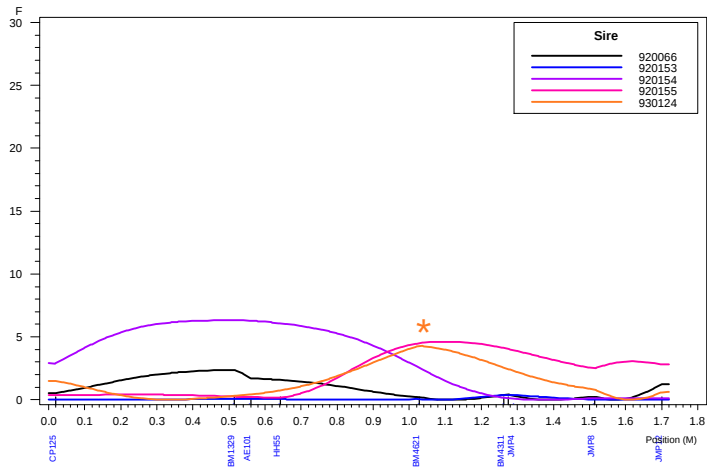
Haley-Knott QTL Analysis: Chromosome 6 LAOST
