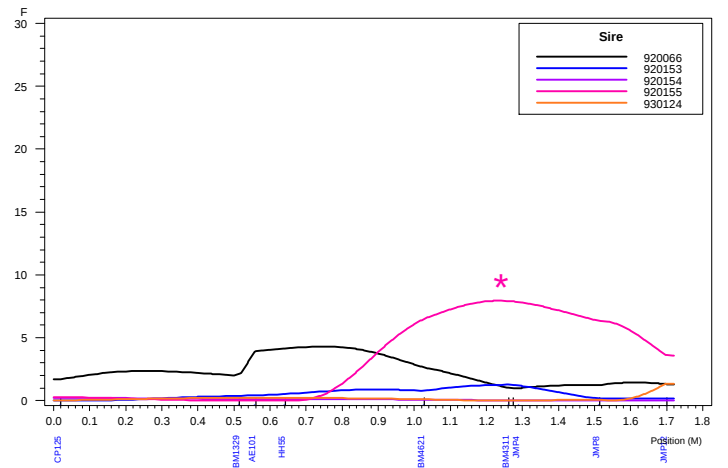
Haley-Knott QTL Analysis: Chromosome 6 WTFEC2
