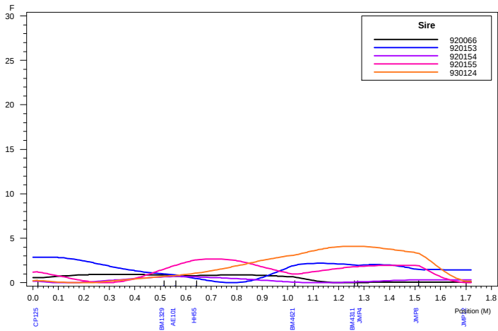
Haley-Knott QTL Analysis: Chromosome 6 ELISA4
