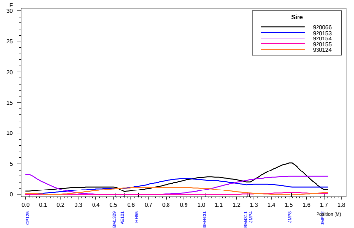
Haley-Knott QTL Analysis: Chromosome 6 DAG1
