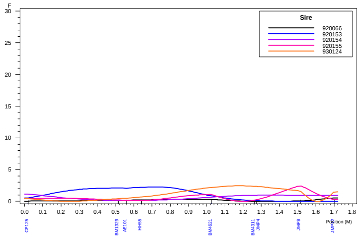
Haley-Knott QTL Analysis: Chromosome 6 DAG0
