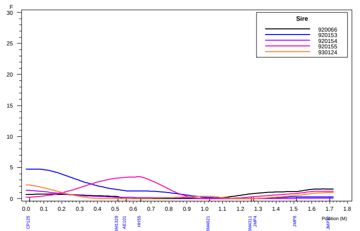
Haley-Knott QTL Analysis: Chromosome 6 ELISA1
