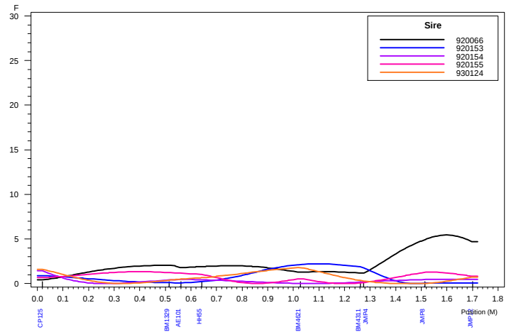
Haley-Knott QTL Analysis: Chromosome 6 LATRICH
