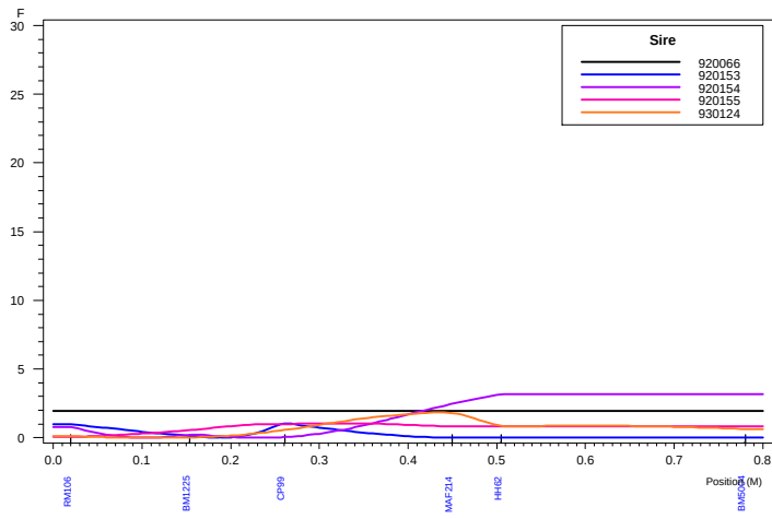
Haley-Knott QTL Analysis: Chromosome 16 SNEM1
