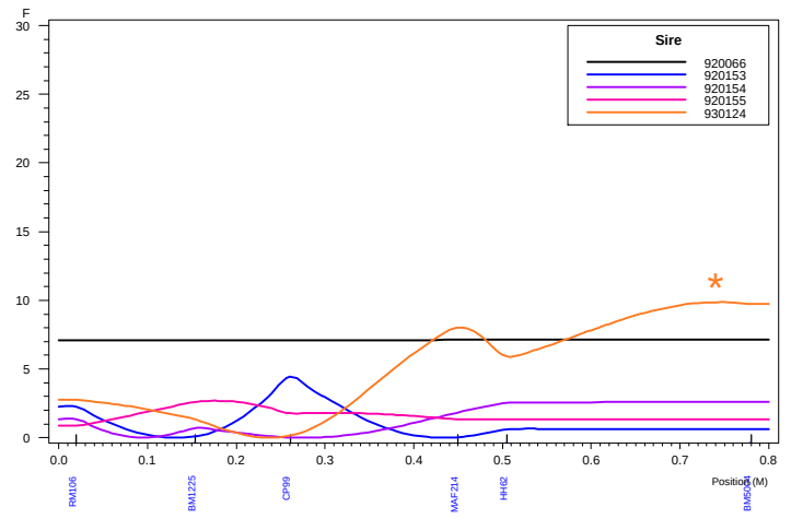
Haley-Knott QTL Analysis: Chromosome 16 SNEM2
