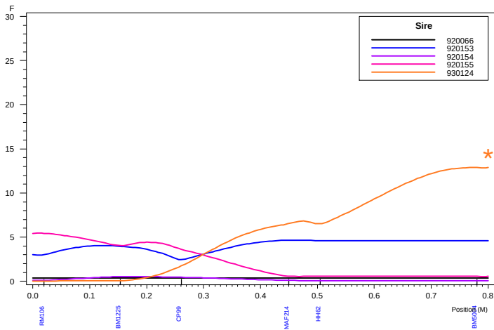
Haley-Knott QTL Analysis: Chromosome 16 LIGE
