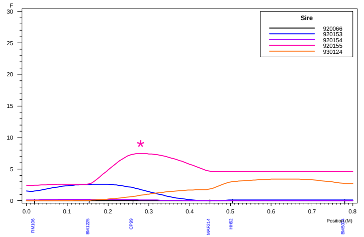
Haley-Knott QTL Analysis: Chromosome 16 ELISA5
