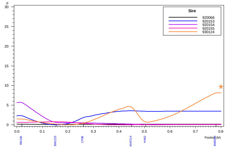
Haley-Knott QTL Analysis: Chromosome 16 DAG1
