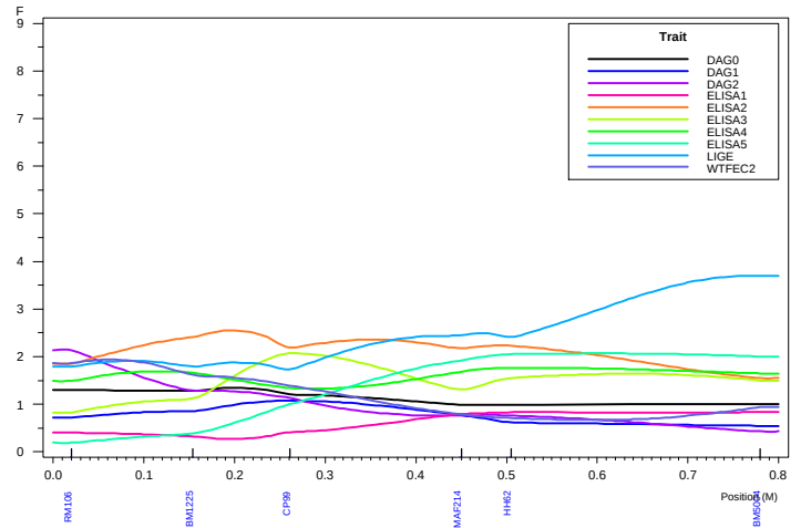
Haley-Knott QTL Analysis: Chromosome 16 LFEC2
