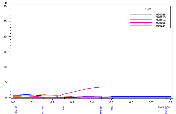
Haley-Knott QTL Analysis: Chromosome 16 ELISA1
