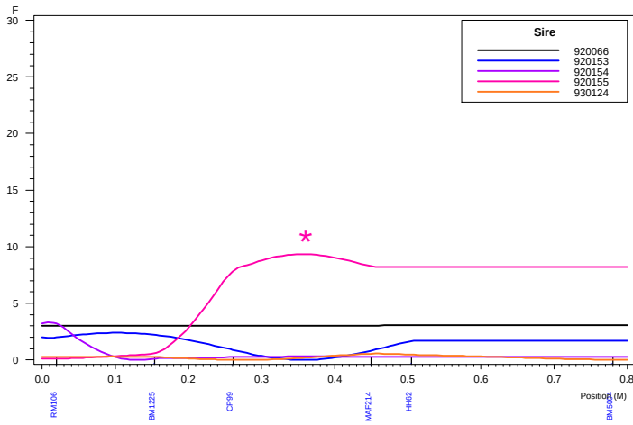
Haley-Knott QTL Analysis: Chromosome 16 LAOST
