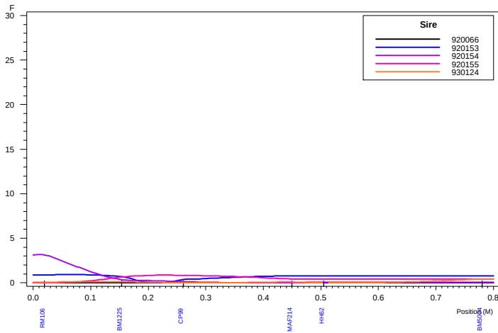
Haley-Knott QTL Analysis: Chromosome 16 DAG0
