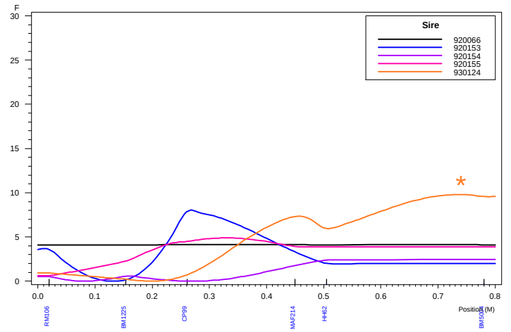
Haley-Knott QTL Analysis: Chromosome 16 LATRICH
