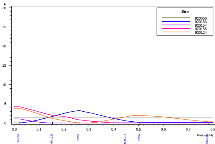
Haley-Knott QTL Analysis: Chromosome 16 DAG2
