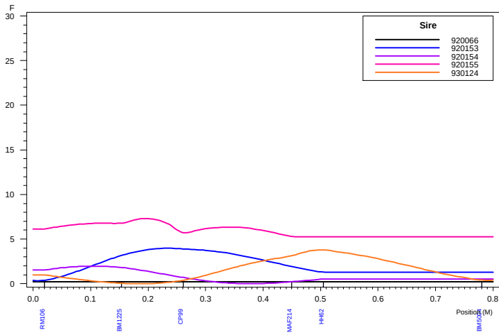
Haley-Knott QTL Analysis: Chromosome 16 ELISA4
