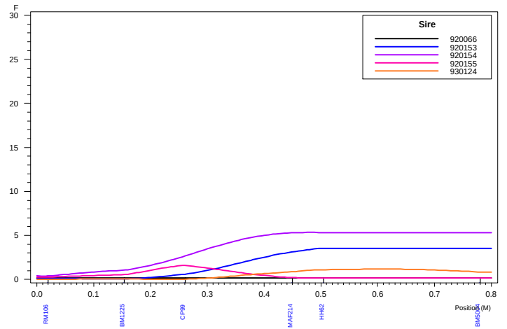
Haley-Knott QTL Analysis: Chromosome 16 WTFEC2
