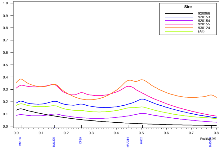
Haley-Knott QTL Analysis: Chromosome 16
