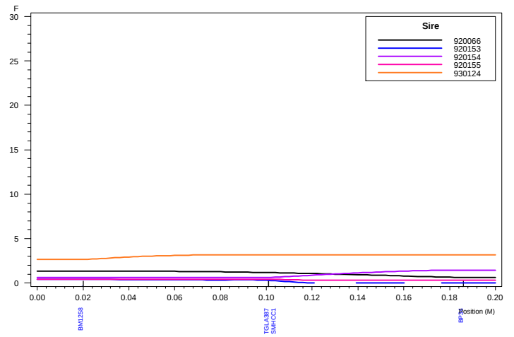
Haley-Knott QTL Analysis: Chromosome 20 ELISA1
