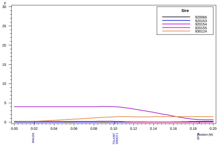
Haley-Knott QTL Analysis: Chromosome 20 DAG0
