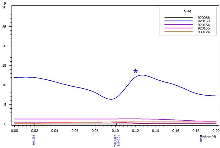
Haley-Knott QTL Analysis: Chromosome 20 LAOST
