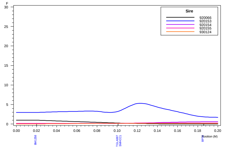
Haley-Knott QTL Analysis: Chromosome 20 ELISA5
