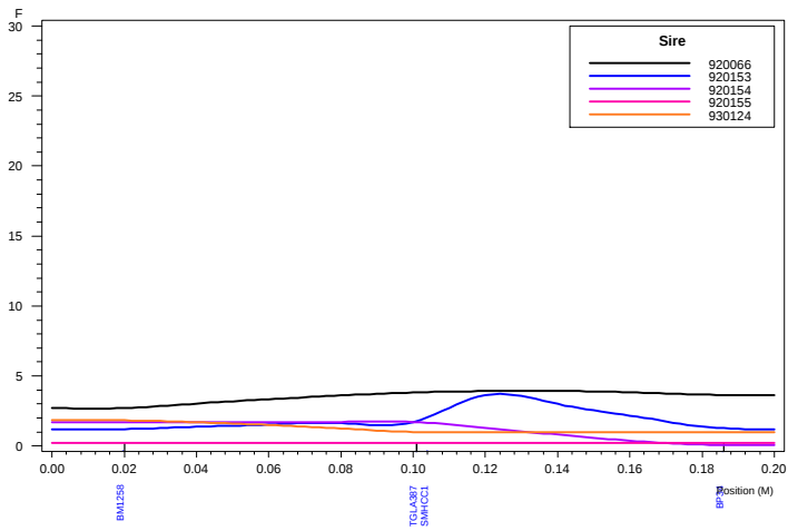
Haley-Knott QTL Analysis: Chromosome 20 LIGE
