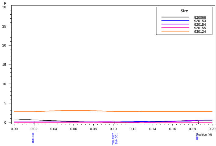
Haley-Knott QTL Analysis: Chromosome 20 ELISA4
