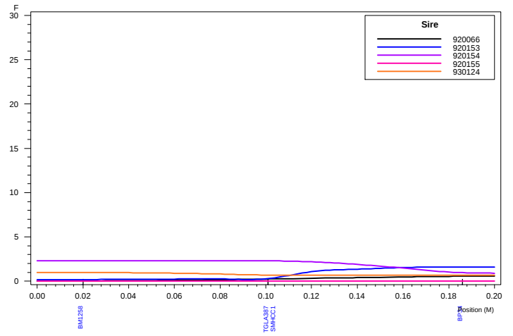
Haley-Knott QTL Analysis: Chromosome 20 WTFEC2
