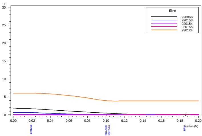
Haley-Knott QTL Analysis: Chromosome 20 DAG2
