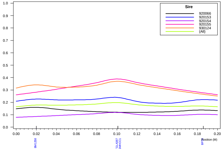
Haley-Knott QTL Analysis: Chromosome 20
