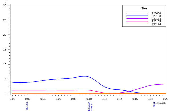
Haley-Knott QTL Analysis: Chromosome 20 LATRICH
