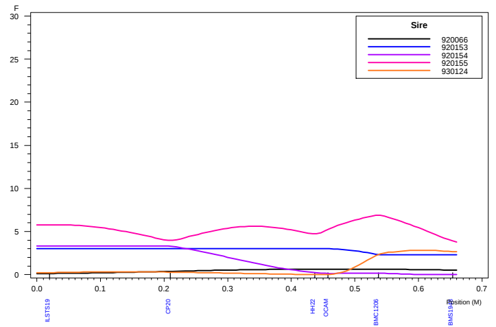
Haley-Knott QTL Analysis: Chromosome 21 ELISA1
