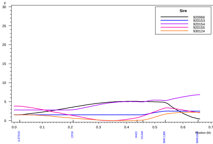
Haley-Knott QTL Analysis: Chromosome 21 LAOST
