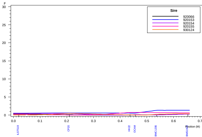
Haley-Knott QTL Analysis: Chromosome 21 DAG2
