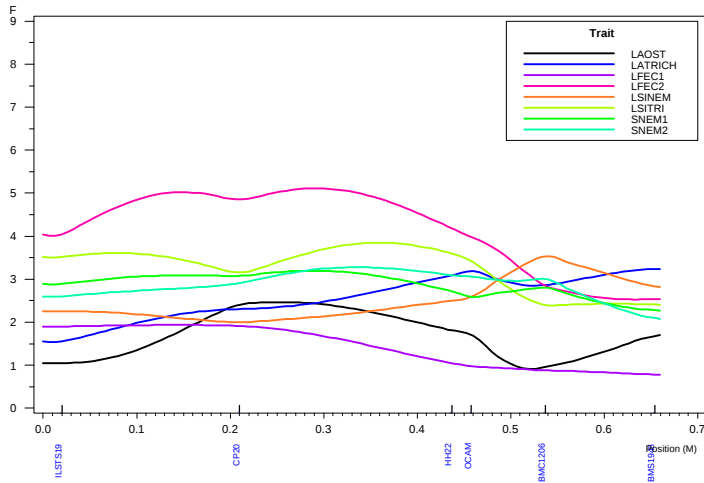
Haley-Knott QTL Analysis: Chromosome 21 LFEC1
