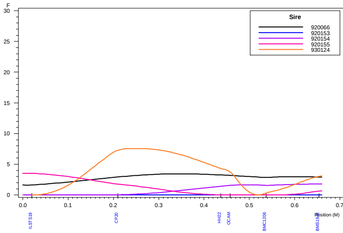
Haley-Knott QTL Analysis: Chromosome 21 DAG0
