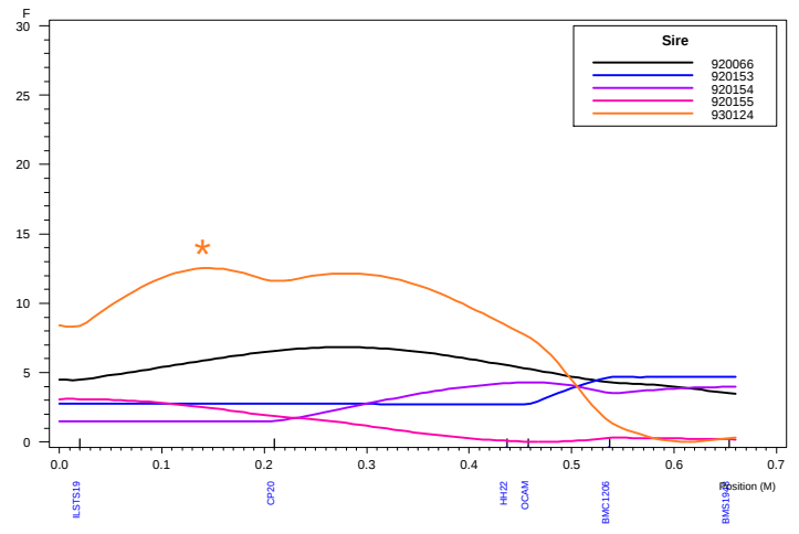
Haley-Knott QTL Analysis: Chromosome 21 SNEM2
