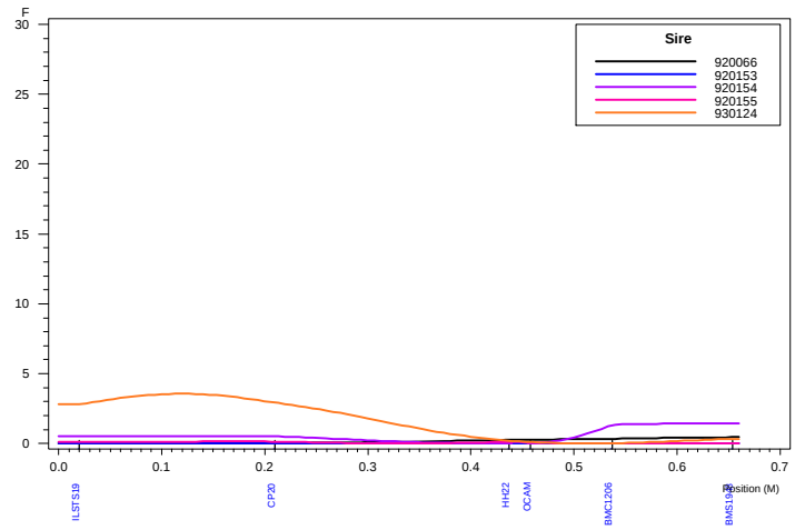
Haley-Knott QTL Analysis: Chromosome 21 WTFEC2
