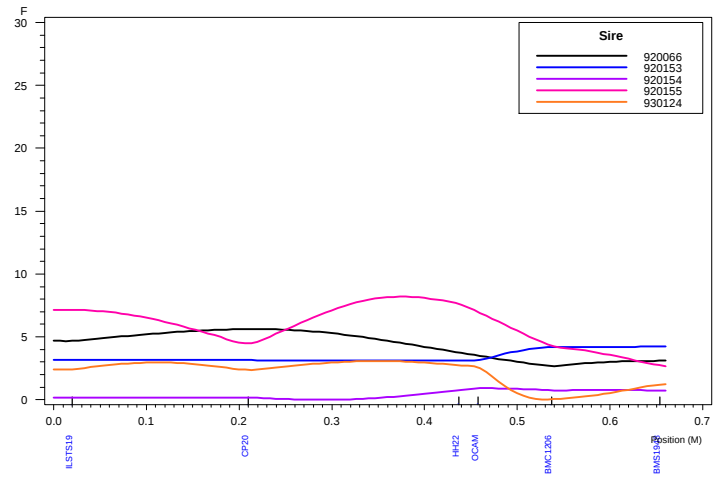
Haley-Knott QTL Analysis: Chromosome 21 LATRICH
