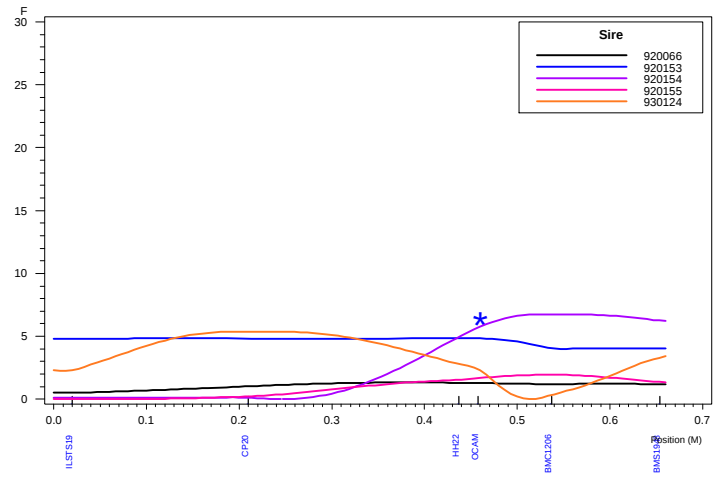
Haley-Knott QTL Analysis: Chromosome 21 DAG1
