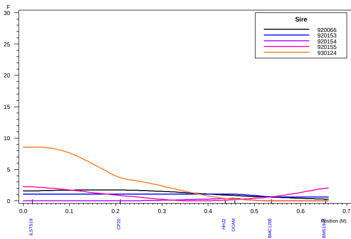
Haley-Knott QTL Analysis: Chromosome 21 LIGE
