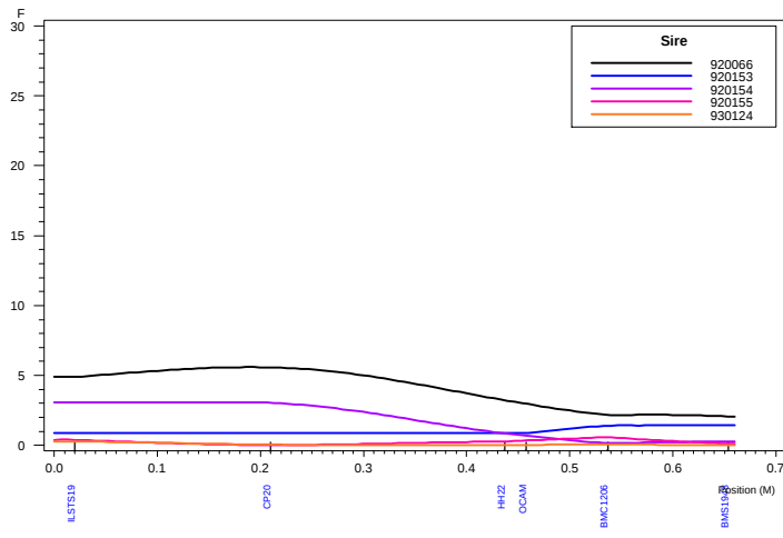
Haley-Knott QTL Analysis: Chromosome 21 SNEM1
