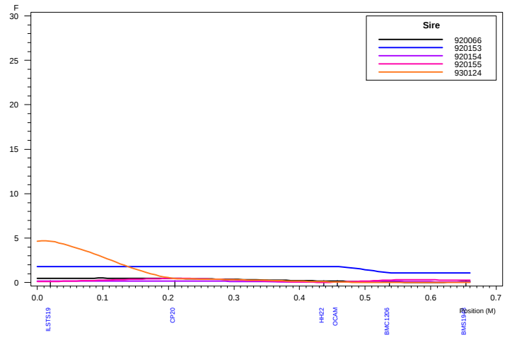
Haley-Knott QTL Analysis: Chromosome 21 ELISA5
