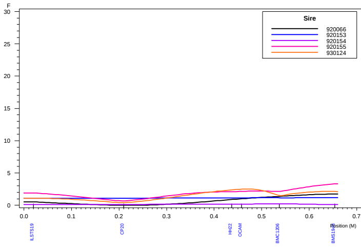
Haley-Knott QTL Analysis: Chromosome 21 ELISA4
