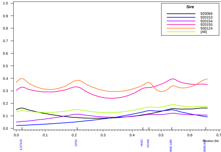
Haley-Knott QTL Analysis: Chromosome 21
