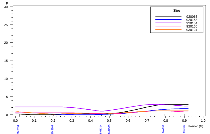
Haley-Knott QTL Analysis: Chromosome 22 WTFEC2
