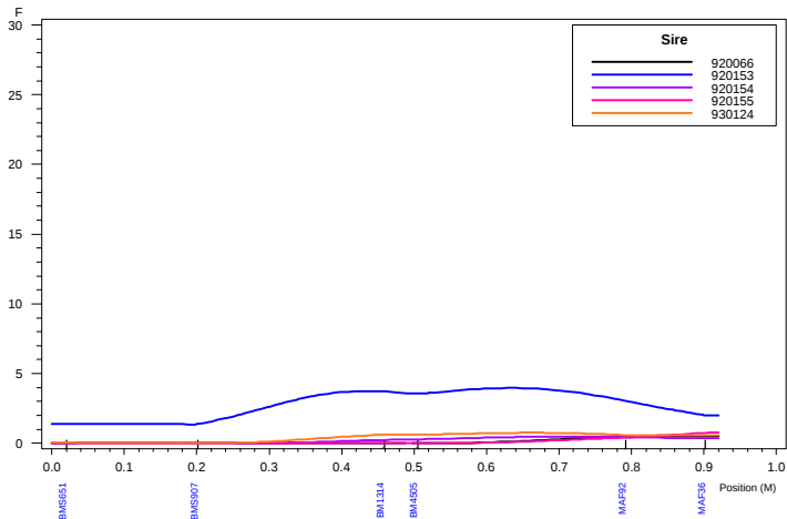
Haley-Knott QTL Analysis: Chromosome 22 LAOST
