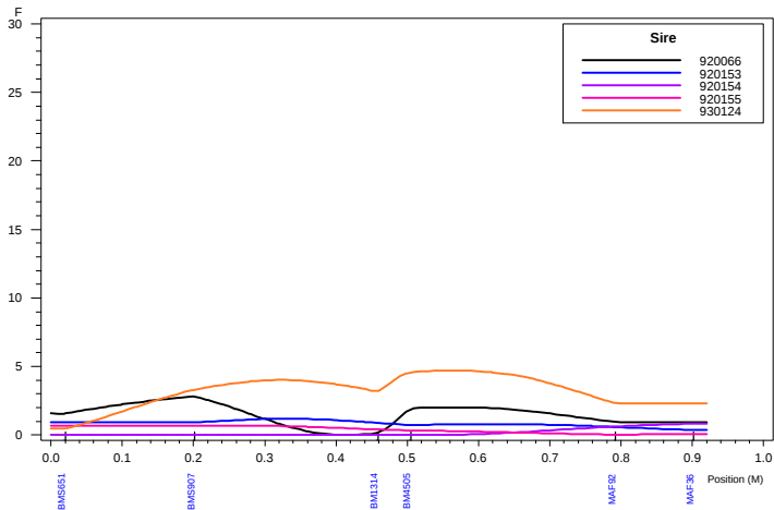
Haley-Knott QTL Analysis: Chromosome 22 LIGE
