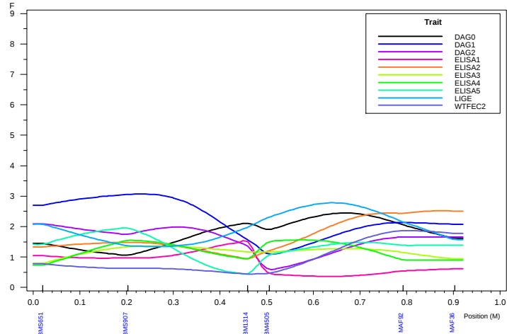
Haley-Knott QTL Analysis: Chromosome 22
