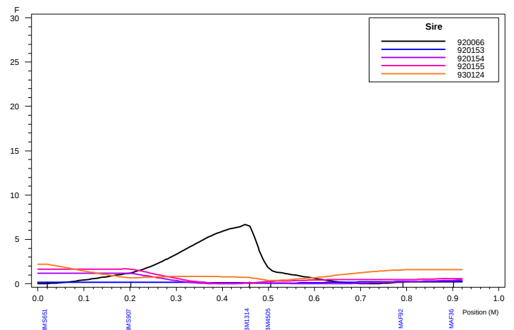
Haley-Knott QTL Analysis: Chromosome 22 ELISA1
