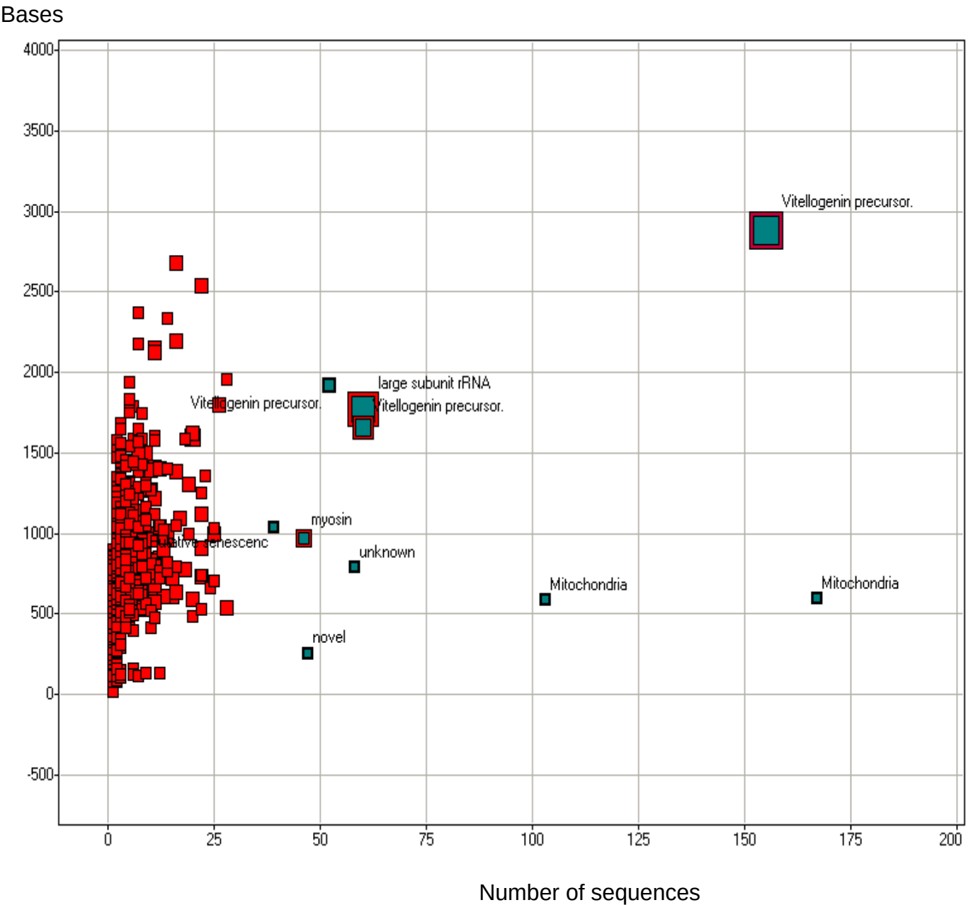
Figure 1. Number of sequences building a contig versus the contig length
