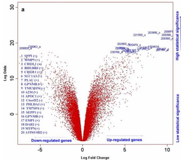
Affymetrix - statistical significance Vs. Fold change
