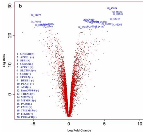
Illumina - Statistical Significance vs Fold Change
