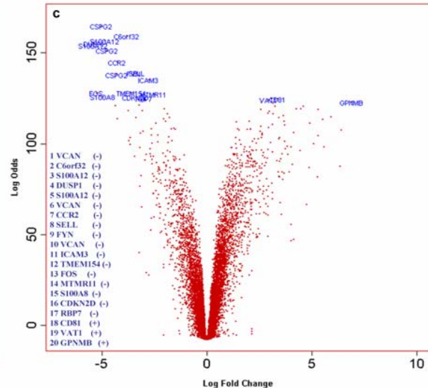
RNG-86 - Statistical Significance vs Fold Change
