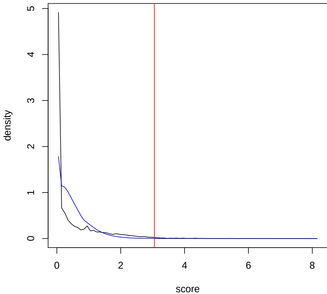
score histogram
