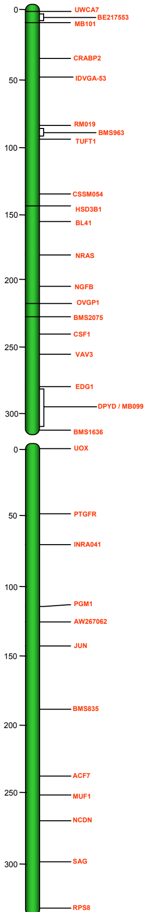
BBU6 - Preliminary RH map (Stafuzza et al. 2007)
