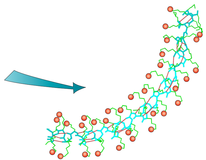
Predicted folding of a helical polylysine segment with peptides attached
