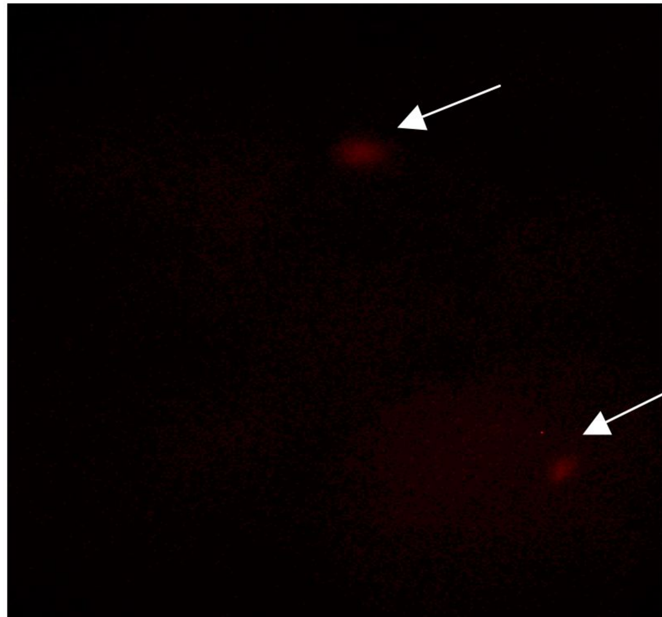
T-Type \text{Ca}^{2+} Channel protein Red
