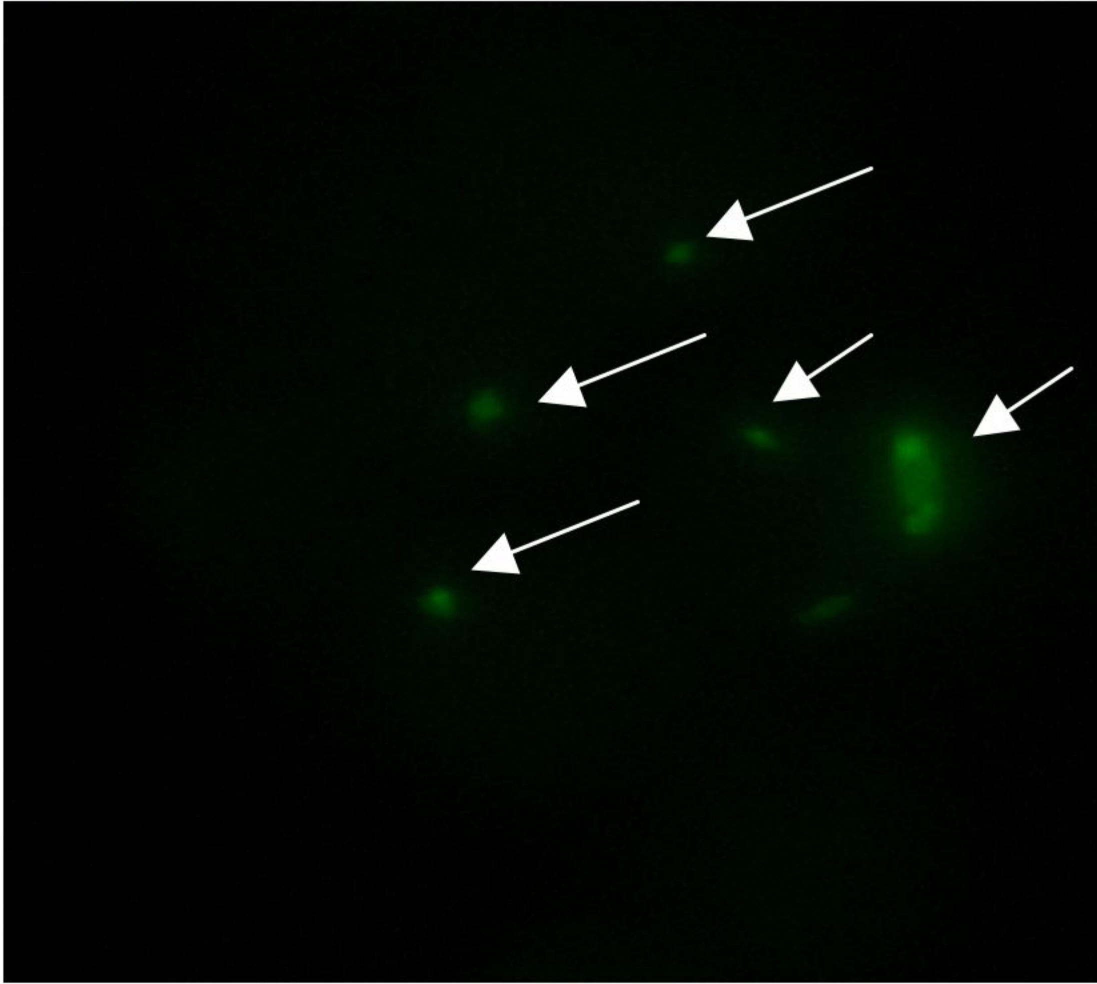
Complemented M. avium 2D6 Mutant Green
