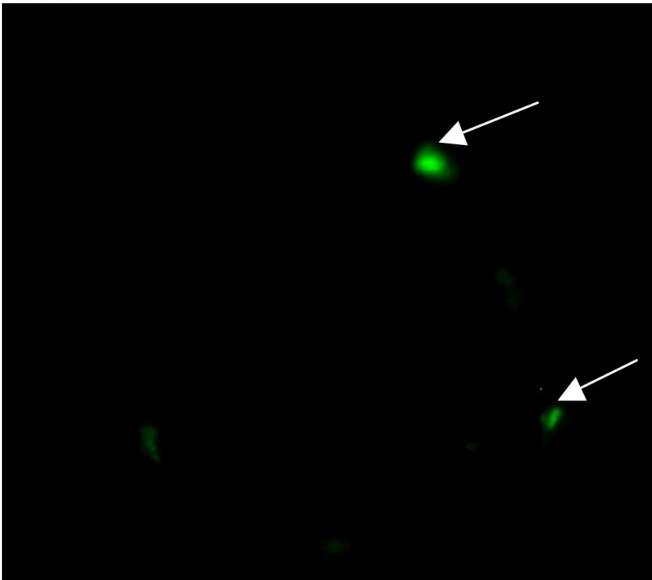
2D6 Mutant Green Positive Control
