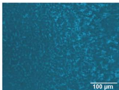
Rt2472 rosR -
