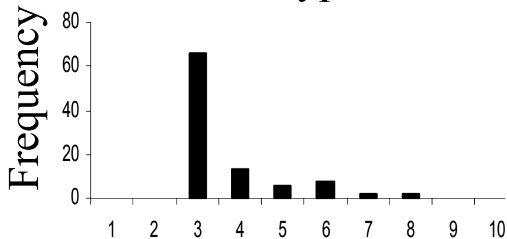
Genotype C
