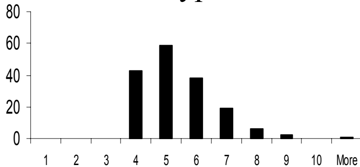
Genotype D
