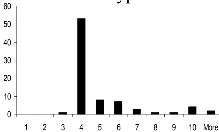
Genotype D
