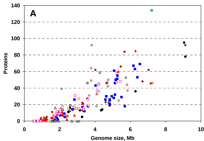
Histidine kinases
