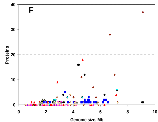
Adenylate cyclases
