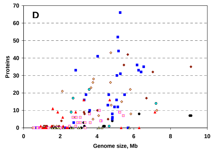
Diguanylate cyclases
