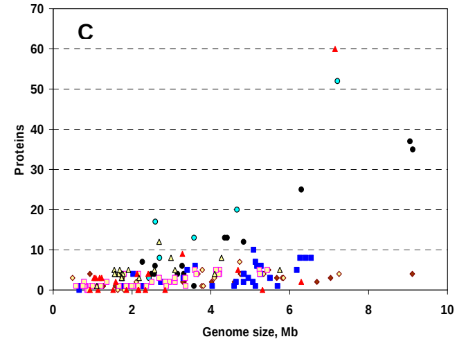
Adenylate cyclases
