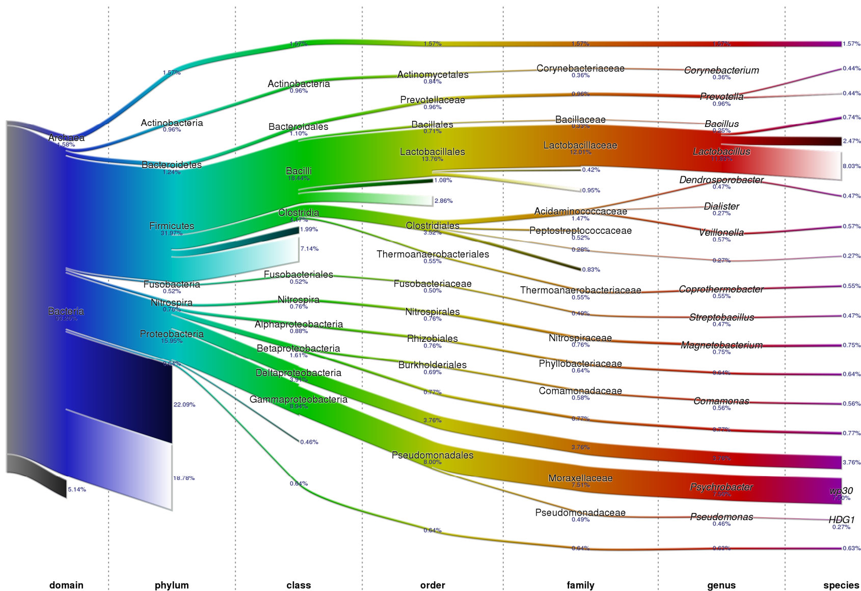
Supplementary Figure S2. Sample B phylogenetic content.
