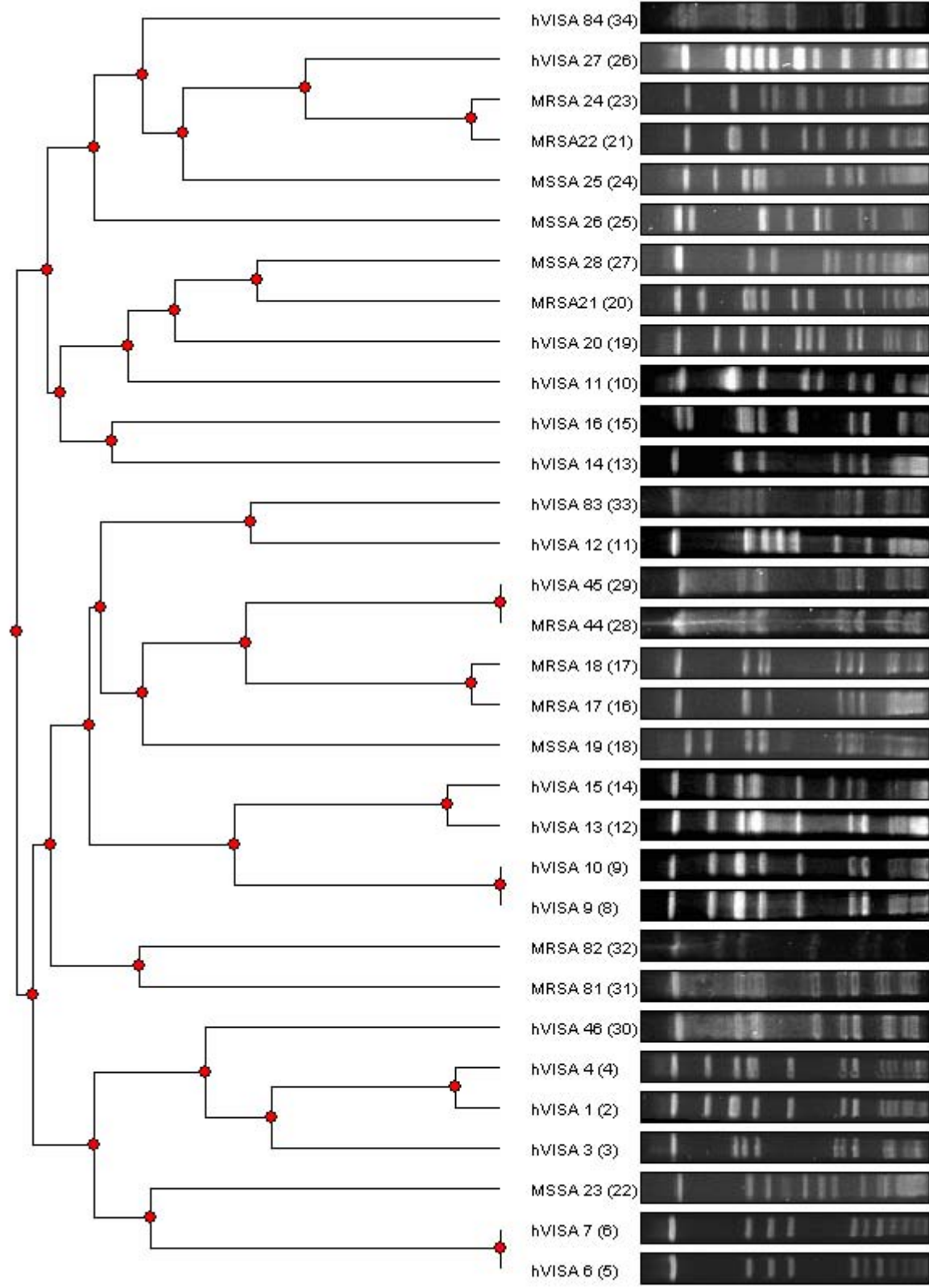
Dice coefficient
