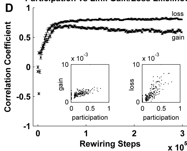
Participation vs Link Gain/Loss Likelihood
