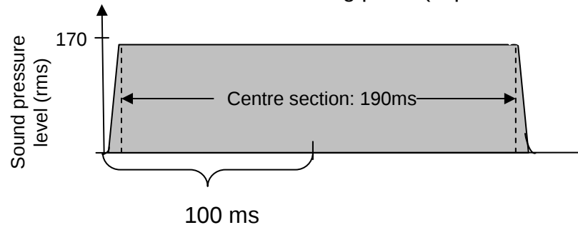
Long rise-time, non-startling pulse (experiment. 3)
