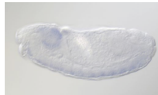
(l) Chrac-16
