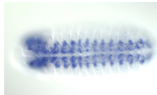
(k) Sd
