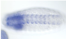
(r) CG5175
