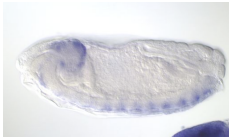
(b) CycB3
