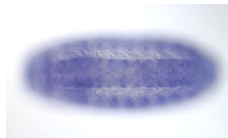
(g) lola
