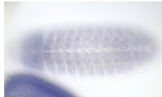
(c) cdc2
