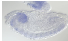
(s) CG8478
