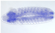
(i) Set
