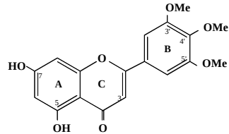
Trimethyltricetin
