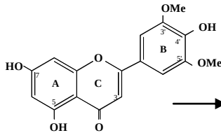
Tricin
