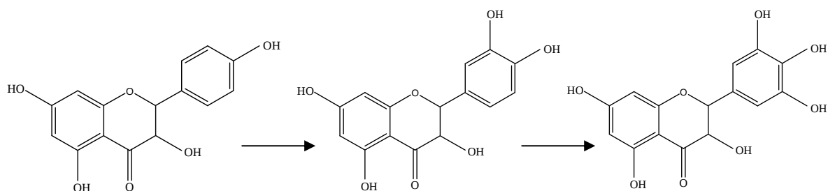
Dihydrokaempferol (3,5,7,4'-tetrahydroxyflavanone)
