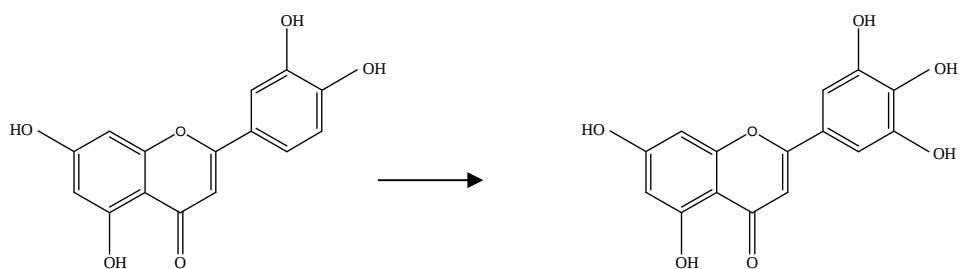
Luteolin (5,7,3',4'-tetrahydroxyflavone)
