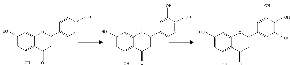
Naringenin (5,7,4'-trihydroxyflavanone)
